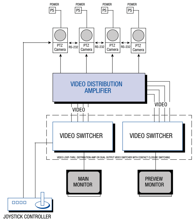
Four camera system setup with Sony Joystick.
